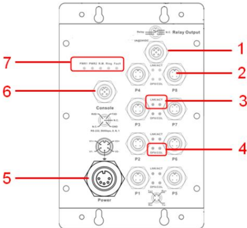
SWMT-80-M12-W/ SWMT-80-M12-W-BP2
